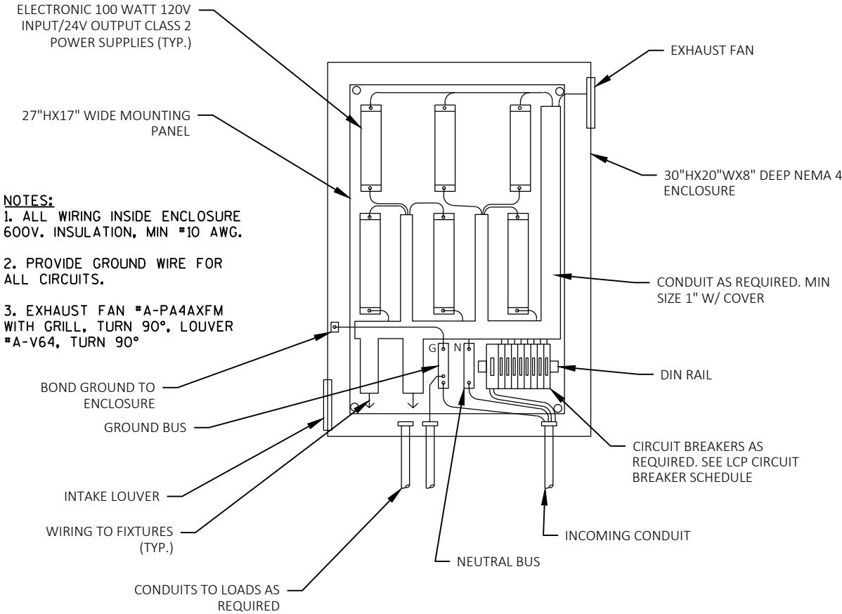
LIGHTING CONTROL PANEL EQUIPMENT DETAIL
