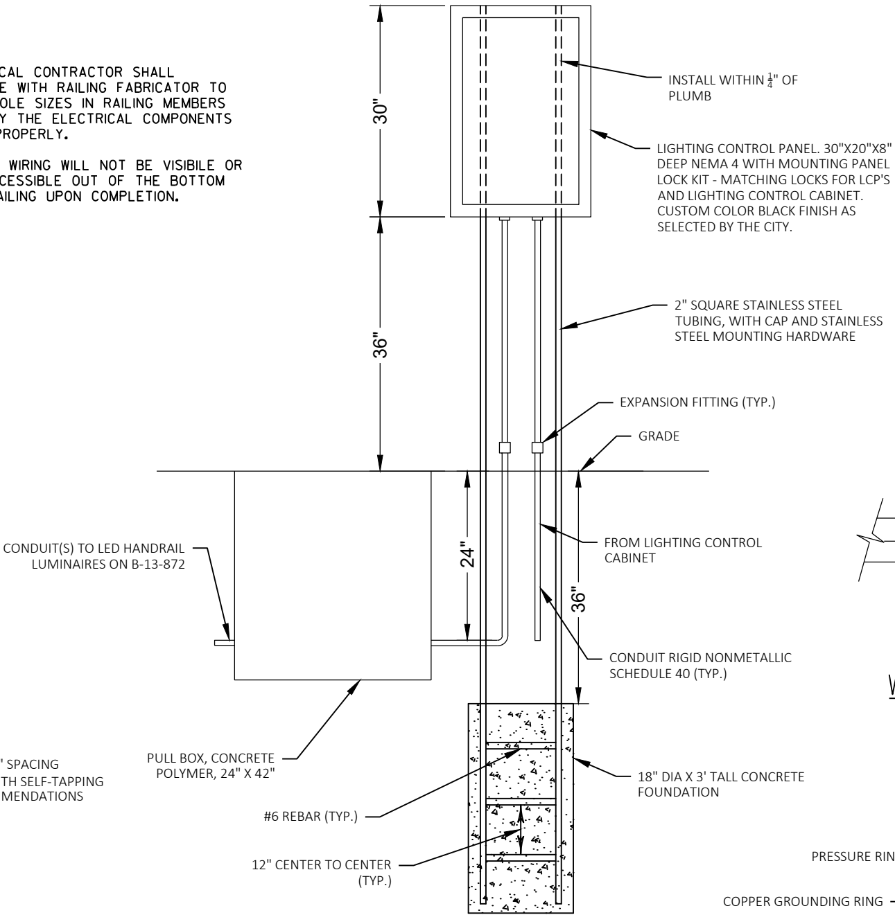
LIGHTING CONTROL PANEL MOUNTING DETAIL
