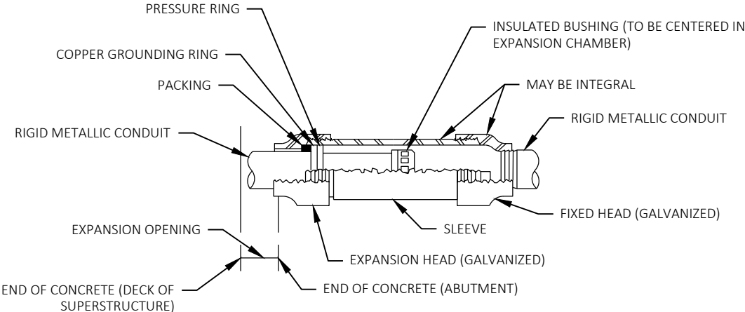
EXPANSION FITTING DETAIL
