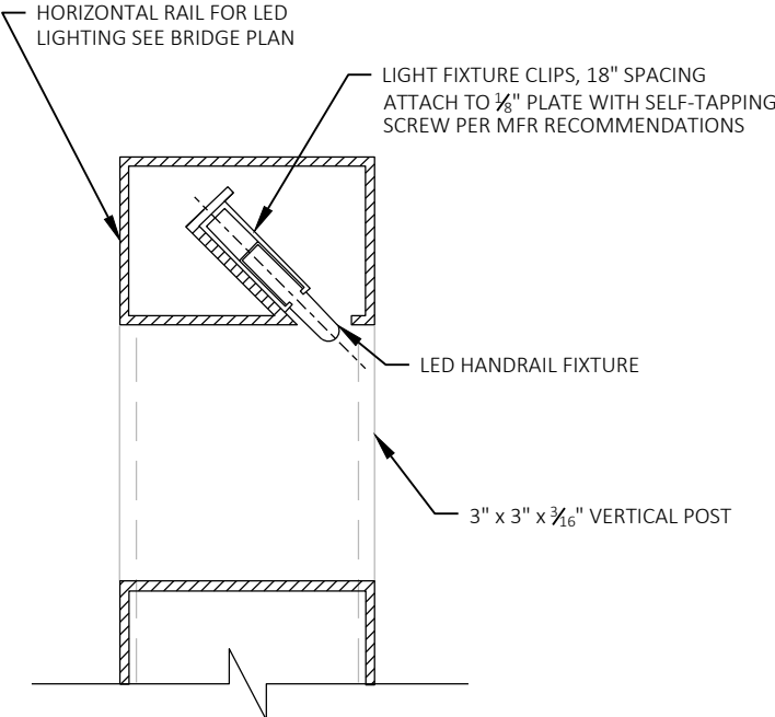
LED HANDRAIL MOUNTING DETAIL
