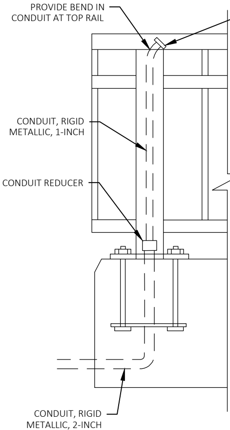
END POST DETAIL
