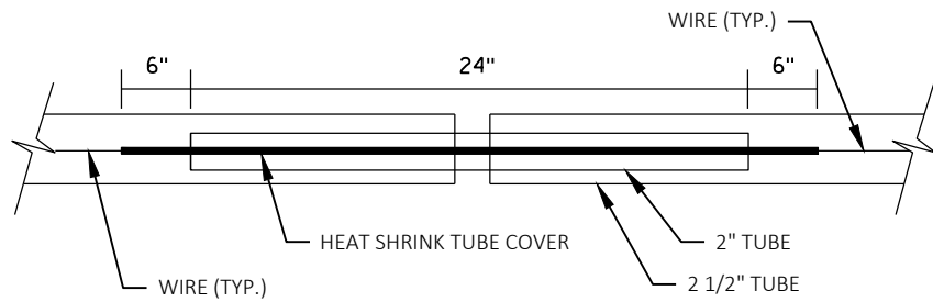
WIRING INSTALLATION AT HANDRAIL EXPANSION JOINT
